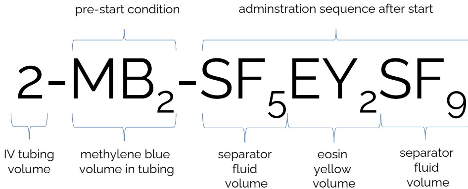
Figure 2. The coding of administration profiles. The three segments (separated by a horizontal line) respectively represent the IV tubing volume in ml, pre-start condition, and the administration sequence. MB: methylene blue, EY: eosin yellow, SF: separator fluid. Numbers trailing the substance indicators in subscript indicate the volume of the indicated substance in ml.
