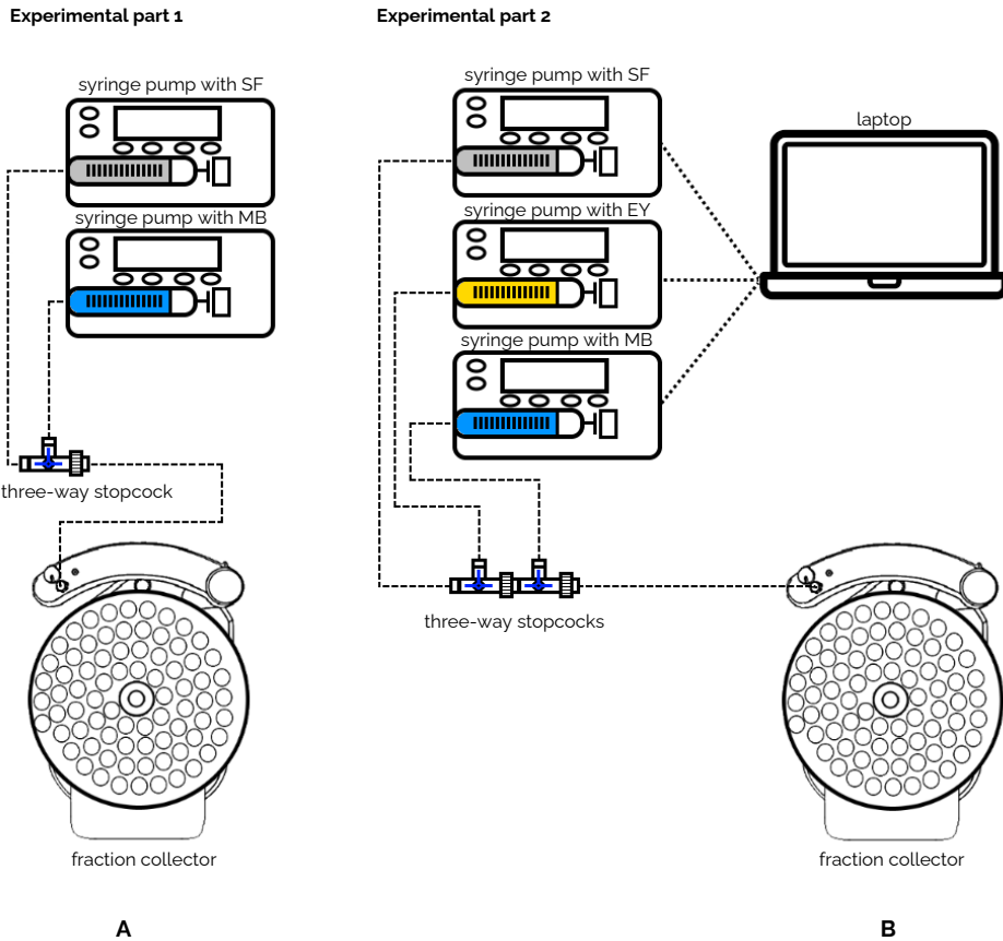
Figure 1. A: Experimental set up used to investigate whether and how the administration rate, solvent and separator fluid (SF) affect the required SF volume (SFV). A 2 meter (2 ml) IV tube runs between the three-way stopcock and the fraction collector. And B: Experimental set up used to investigate whether and how IV line volume affects the required SFV in different administration profiles. MB: methylene blue, EY: eosin yellow. Depending on the administration profile, either a 2 meter (2 ml) IV tube or 2x2 meter tubes (4 ml) run between the stopcocks and the fraction collector.
