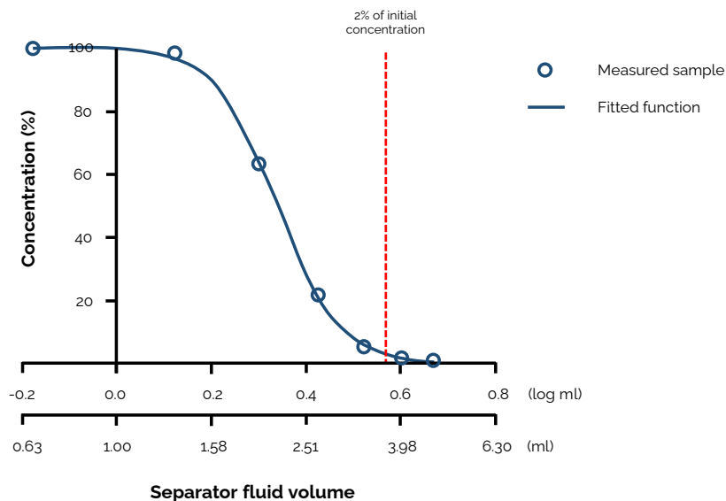
Figure 3. Determination of the separator fluid volume (SFV) at 2% of the initial dye concentration (dashed line). Sample data (circles) were transformed to a logarithmic scale to enable curve fitting (continuous line). The resulting equation was used to obtain the log ml SFV at the 2% concentration, which in turn was transformed back to ml.
