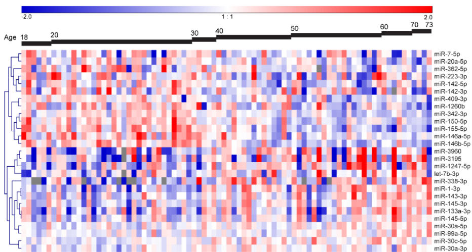
Figure 2. Age-related miRNAs in human bronchial biopsies. Heatmap of the supervised hierarchical clustering of the 27 age-related miRNAs. The 82 subjects were ordered by age. The heatmap shows the median-centred expression of the 27 miRNAs of which 14 miRNAs were higher expressed and 13 miRNAs were lower expressed with increasing age (FDR adjusted p -value <0.05 ).
