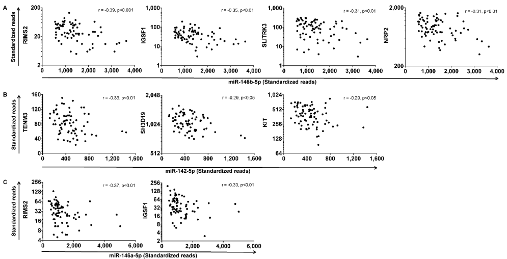
Figure 4. Correlation between miRNA expression and expression of their age-related predicted targets. Lower expressed miRNAs with increasing age, (A) miR-146b-5p, (B) miR-142-5p and (C) miR-146a-5p correlated with their predicted target genes that are higher expressed with age. Spearman's correlation coefficient r and p -values are shown in the graphs.
