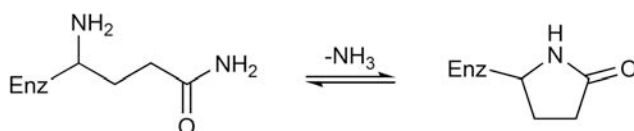
Figure 3. Formation of pyroglutamate (i.e., 5-oxoproline) by deamination of an amino-terminal glutamine.
