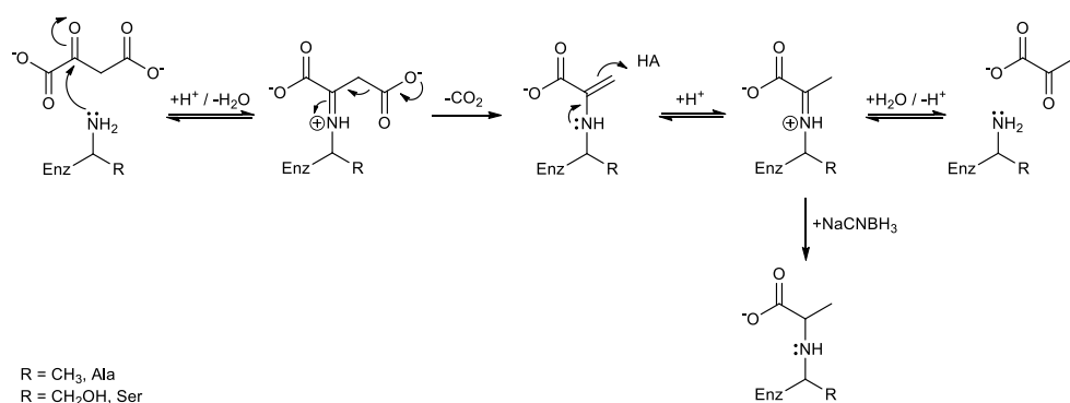
Figure 2. Proposed mechanism of the 4-OT P1A and 4-OT P1S catalyzed decarboxylation of oxaloacetate involving a covalent imine intermediate, which can be trapped using NaCNBH 3 .
