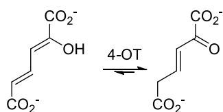
Figure 1. The 4-OT-catalyzed tautomerization of 2-hydroxyhexa-2,4-dienedioate to 2-oxo-hex-3-enedioate.
