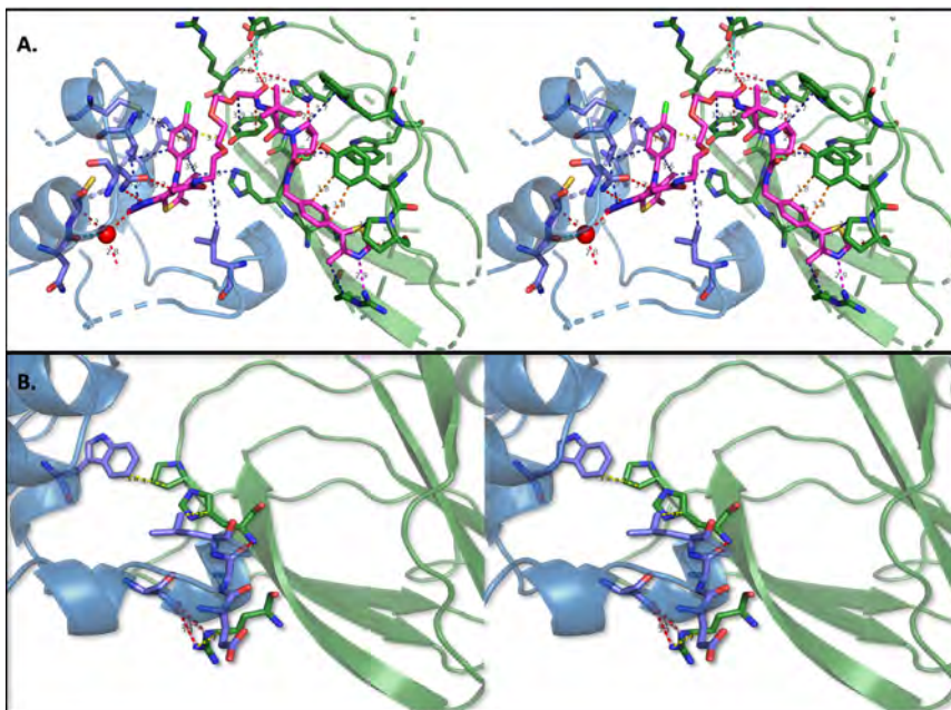
Figure 3. A) Stereo view of ligand – protein interactions between MZ1 (magenta sticks) with BRD4 (blue cartoon), pVHL (green cartoon): hydrogen bonds (red dashes), cat_dip (magenta dashes), dipolar (cyan dashes), hdon_pi (yellow dashes), vdW (dark blue dashes), pi_pi (orange dashes). The key aminoacids participating in the interactions are shown in sticks, B) Stereo view of protein – protein interactions between BRD4 (blue cartoon), pVHL (green cartoon):H bonds as red, ionic as pink and van der Waals as yellow dashes. The key aminoacids participating in the interactions are shown in sticks. The figure was prepared by using Scorpion (Desert Scientific Software, http://saas1.desertsci.com/ ) and Pymol (The PyMOL Molecular Graphics System, Version 2.0 Schrödinger, LLC).
