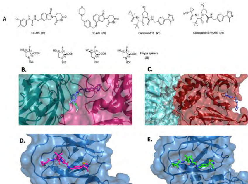
Figure 4. A) Chemical structures of CC-885 ( 19 ), CC-220 ( 20 ), compound 10 ( 21 ) and compound 15 (VH298) ( 22 ) and F-Hyps epimers ( 23 ), B) Crystal structure of CC-885
