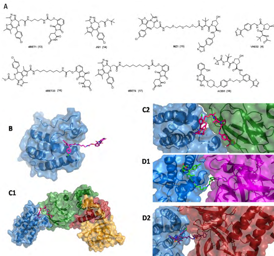
Figure 2. A) structures of dBET1 PROTAC ( 13 ), JQ1 ( 14 ) (BET inhibitor), MZ1 PROTAC ( 15 ), VH032( 4 ) (VHL inhibitor), dBET23 PROTAC ( 16 ), dBET6 PROTAC ( 17 ) and ACBI1 PROTAC ( 18 ), B) Binary complex of dBET1 (purple sticks) with BRD4 (blue surface) [PDB 4ZC9], C1) Ternary complex of MZ1 (magenta sticks) with BRD4 (blue surface), pVHL (green surface), elongin C (red surface), elongin B (gold surface) [PDB 5T35], C2) closeup view BRD4 (blue surface) - MZ1 (magenta sticks) - pVHL (green surface), D1) Ternary complex of dBET23 (green sticks) with BRD4 (blue surface) and CRBN (magenta surface) [PDB 6BN7], D2) Ternary complex of dBET6 (purple sticks) with BRD4 (blue surface) and CRBN (red surface) [PDB 6BOY].The figure was prepared in Pymol (The PyMOL Molecular Graphics System, Version 2.0 Schrödinger, LLC).
