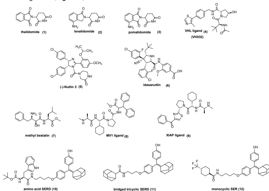
Figure 1. Structures of E3 ligase degraders.
