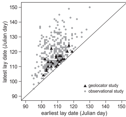
Figure 6.3. Individual consistency of lay date observed in our geolocator and observational studies. Here, we plotted the earliest lay date versus the latest lay date for every individual with repeated measurements for lay date. We also plotted the line x=y , which represents a scenario in which lay date is completely consistent, i.e. 100% repeatable. The observed difference in consistency between the two study methods has consequences for the estimated individual repeatability.
