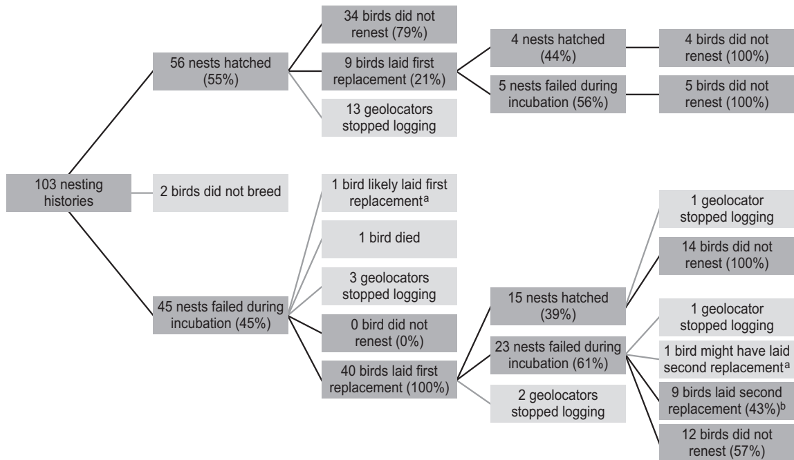
Figure 6.2. Flowchart of all complete and incomplete incubation histories collected with geolocators. Terminology used is defined in Materials and Methods. That geolocators stopped logging (including the retrieval of a geolocator during one breeding season, but not in a subsequent breeding season; see Materials and Methods) resulted in incomplete histories (light grey boxes); the presented percentages are based on complete histories only (dark grey boxes). As a result, the sum of dark grey boxes originating from the same dark grey box is always 100%. a see Materials and Methods for explanation. b of these 9 second replacement clutches, 7 failed (88%), 1 hatched (12%) and 1 stopped logging.
