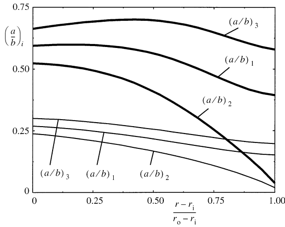
Fig. 8. Distribution of cavitation damage, expressed in (a/b)_i , along the vessel wall in case of the constitutive relations without rigid grain mode cavitation: thin lines, after 28 years; thick lines, at failure after 219 years.
