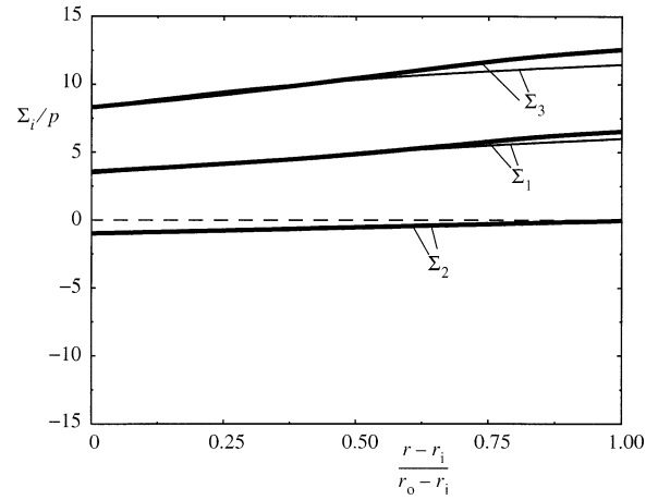
Fig. 10. Macroscopic stress distribution after 28 years (thin lines) and after 219 years (thick lines).
