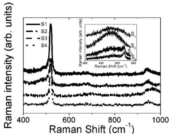
Figure 4 Raman spectra of the films annealed at 900 °C; the insert displays the spectra of the films annealed at 800 °C.
