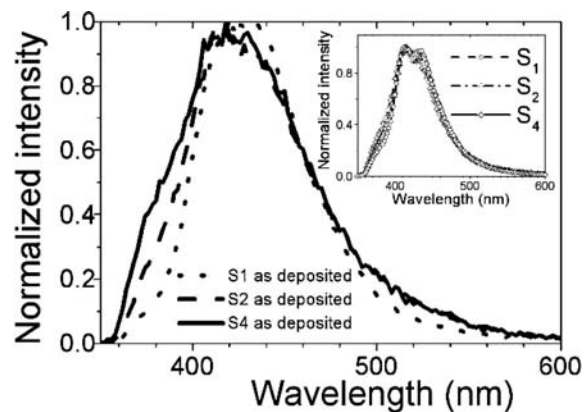
Figure 5 Typical room temperature PL spectra observed in the films as deposited; the insert displays the spectra of the annealed films at 800 °C.
