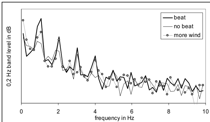
Figure V.6: sound power spectrum of A-weighted broad band immission sound level at façade of dwelling P when beating is distinctly or not audible and with slightly increased wind speed. The ordinate spans 20 dB.
