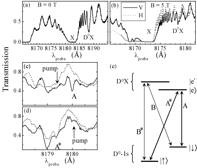
Figure 6.1: (a) Transmission spectroscopy at B = 0 T. (b) Transmission at B = 5.0 T for H and V polarization. (c) Pump-assisted spectroscopy with H-polarized pumping at the A^* transition shows enhanced absorption for the A transition for the scan with a V-polarized probe (solid line), but not with an H-polarized probe (dashed trace). (d) Complementary to (c), V-polarized pumping at A shows enhanced absorption for the A^* transition with an H-polarized probe. (e) Energy levels and optical transitions of the D^0 - D^0X system.
