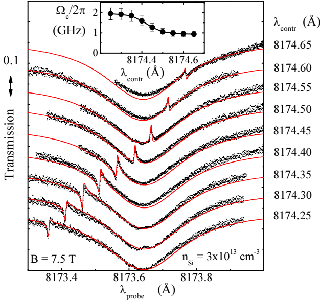
Figure 6.3: Dependence of EIT spectra on control-field detuning. The position of the EIT peak follows precisely the control-field detuning from transition A. Dots - experiment with control (probe) intensity 6 (0.04) \text{Wcm}^{-2} . Lines - fits with T_2^* = 2 \text{ ns} and \Omega_c as presented in the inset.
