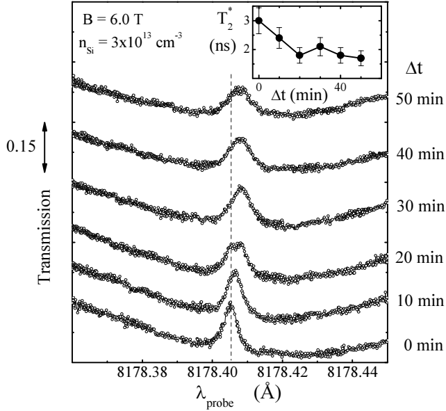
Figure 6.4: Evolution of the EIT peak after 30 min pumping of the A^* transition. Fast EIT ‘snapshots’ were taken at 10 min intervals during which the sample was kept in the dark. The dashed line is a guide for showing the shift in peak position. The inset presents fitting results that show the change in T_2^* .
