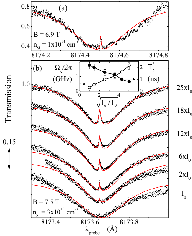
Figure 6.2: (a) EIT spectrum from sample with Si doping at 1 \times 10^{14} \text{ cm}^{-3} . Dots - experiment. Line - numerical fit. (b) EIT spectra from sample with Si doping at 3 \times 10^{13} \text{ cm}^{-3} , for probe-field intensity 0.04 \text{ Wcm}^{-2} and a range of control-field intensities I_c with I_0 = 0.4 \text{ Wcm}^{-2} . The inset shows the fitting results for Rabi frequency \Omega_c and spin dephasing time T_2^* .
