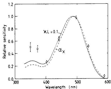
Fig. 3. The mean spectral sensitivity of visual pigment poor R1-6 photoreceptor cells of chalkies, reared on a vitamin A deprived diet and kept under light conditions with no blue light. The dotted curve is the normalized absorption spectrum of blowfly visual pigment (Schwemer, 1979). The continuous curve is the best fit of the mean spectral sensitivity, calculated from equation (1) of the Methods. The mean sensitivity in the U.V. differs from the calculated fit, presumably because some sensitizing pigment is present.
