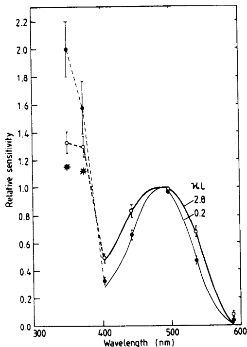
Fig. 4. The mean spectral sensitivity of R1-6 photoreceptors of wild type blowflies. All flies were reared on a vitamin A rich diet. One group of flies was reared under light conditions with no blue light (dots); the other group with blue light (open circles). The best fits in the visible band, calculated from equation (1) (Methods) are also shown (continuous lines). Note the difference in broadening of the curves in the visible band, which is due to selfscreening. Assuming that in both cases the ratio sensitizing pigment/visual pigment is maximal the relative U.V. sensitivity in the visual pigment rich cells has been calculated from the values of the pigment poor cells using equation (2) (Methods) and assuming \gamma_s = 1 (asterisks). The measured relative U.V. sensitivities of the visual pigment rich flies differ only slightly from the calculated values.
