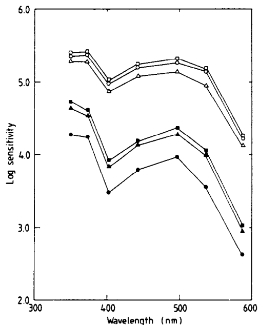
Fig. 1. Two sets of spectral sensitivity curves; wild type blowflies. Each set of curves is obtained from visual sense cells of one fly. The upper set of curves are measured from cells of a visual pigment rich fly (vitamin A rich diet and normal daylight). The lower set of curves are measured from cells of a visual pigment poor fly (vitamin A rich diet and held under light conditions with no blue light). Note the differences in absolute sensitivity, in broadening of the curve in the visible band and in relative U.V. sensitivity.
