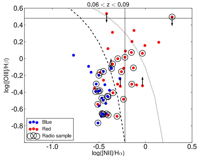
Figure 2.2: BPT diagram of 26 blue (SF+LINER) and 31 red (SF+LINER) Lockman Hole galaxies with SDSS spectra available in the highest redshift bin. Arrows mark the limits for galaxies for which only three optical lines are measured above S/N > 2 (in the other galaxies all four lines have S/N > 2 ). The vertical and horizontal lines represent the conventional separation for LINERs (i.e. [[\text{O III}]]/\text{H}\beta < 3 and [[\text{N II}]]/\text{H}\alpha > 0.6 ) and Seyfert galaxies (i.e. [[\text{O III}]]/\text{H}\beta > 3 and [[\text{N II}]]/\text{H}\alpha > 0.6 ). In this work we adopt the demarcation by Kauffmann et al. (2003) ( dashed line ) to separate star-forming galaxies from LINERs. The dotted line indicates the more stringent demarcation to identify AGN, proposed by Kewley et al. (2001). The radio subsample is marked by circles (31 sources). This figure excludes the inactive galaxies, see Sec 2.5.2 for more detail.
