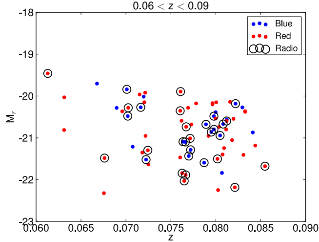
Figure 2.4: Magnitude of the blue (26) and red (47) galaxies in the highest redshift bin. Circles indicate radio detected objects.
