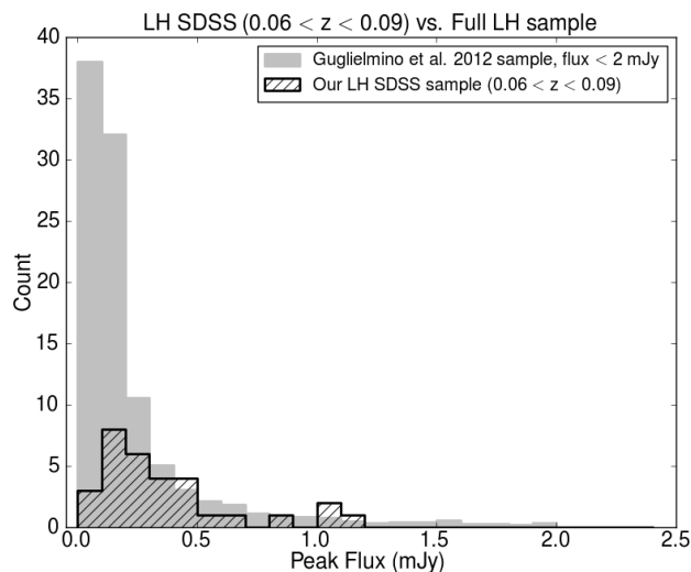
Figure 2.3: Flux distribution of the highest redshift radio sample used in this study ( black hatched region , i.e. 31 radio sources with available SDSS redshift) compared to the distribution of the entire radio sample in the Lockman Hole ( grey area , Guglielmino et al. 2012). For the Guglielmino et al. (2012) sample, sources with larger fluxes are also found, however here we only plot sources with peak flux < 2 mJy, in order to match the distribution of sources in this study. The latter distribution is normalized by the total number of galaxies (below 2 mJy) detected in the catalog of Guglielmino et al. 2012. The radio power corresponding to the fluxes is \log(P_{1.4\text{GHz}}) < 22.5 \text{ W Hz}^{-1} .
