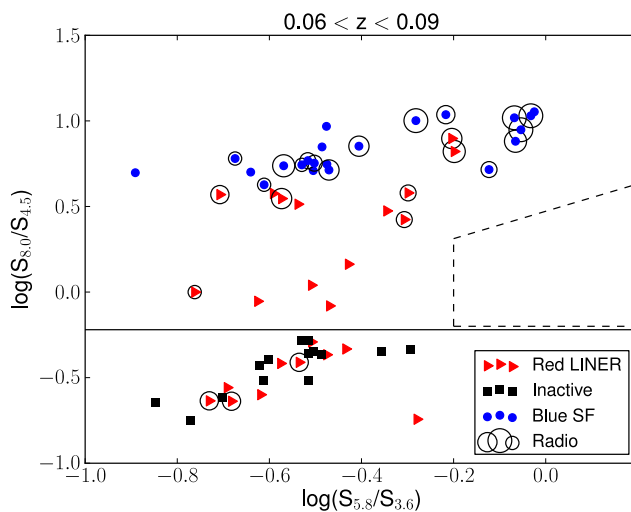
Figure 2.8: Infrared color-color plot in the highest redshift bin for galaxies with Spitzer detection (22 blue SF, 24 red LINER and 14 inactive galaxies). Circles are proportional to the radio power distribution. The dashed line indicates the region for powerful AGN.
