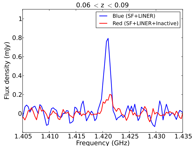
Figure 2.6: HI spectra obtained for blue and red galaxies.
