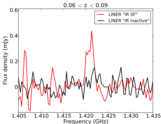
Figure 2.9: HI spectra obtained for LINERs found in the IR SF (red line) and IR inactive (black line) region.
