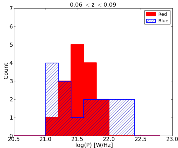
Figure 2.5: Distribution of radio power for blue (16) and red (15) galaxies with radio counterparts in the highest redshift bin.
