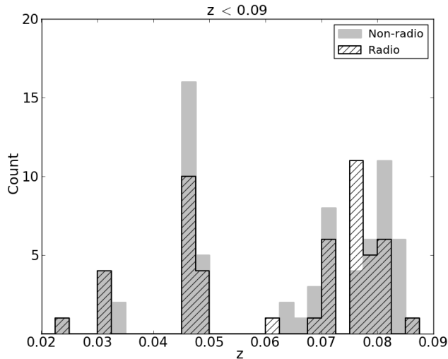
Figure 2.1: Redshift distribution of the SDSS galaxies in the Lockman Hole region, used for our HI stacking experiment
