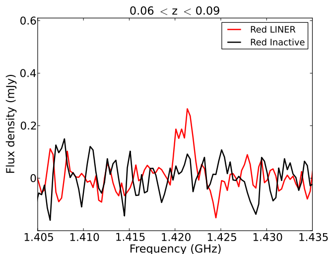
Figure 2.7: Stacked spectra of red LINERs ( red line ) and red inactive galaxies ( black line )
