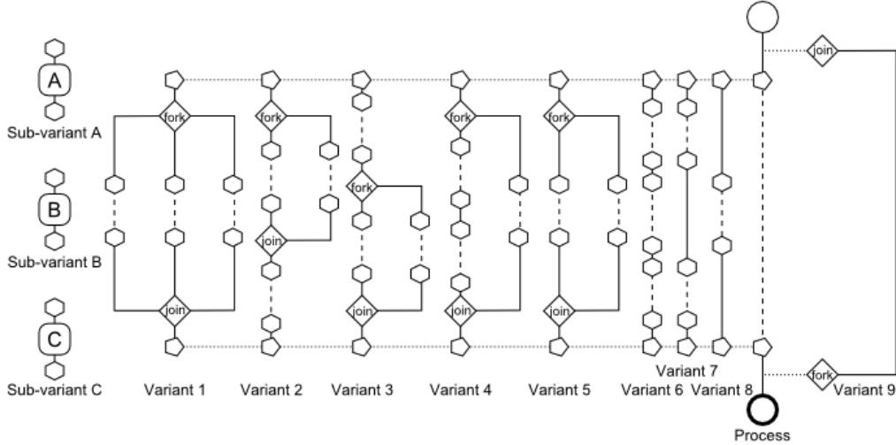
Figure 12: High variable imperative solution.
