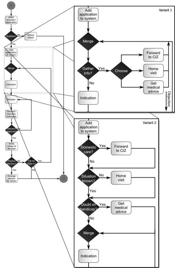
Figure 2: Imperative view on variability within the WMO processes.
