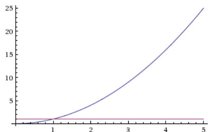
(a) Low variable case with constant (1) imperative and N^2 declarative complexity
