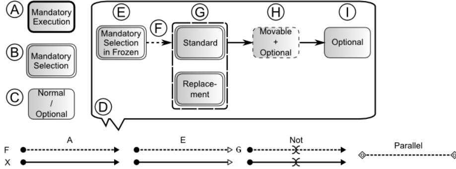
Figure 7: PVDI Graphical Elements.
