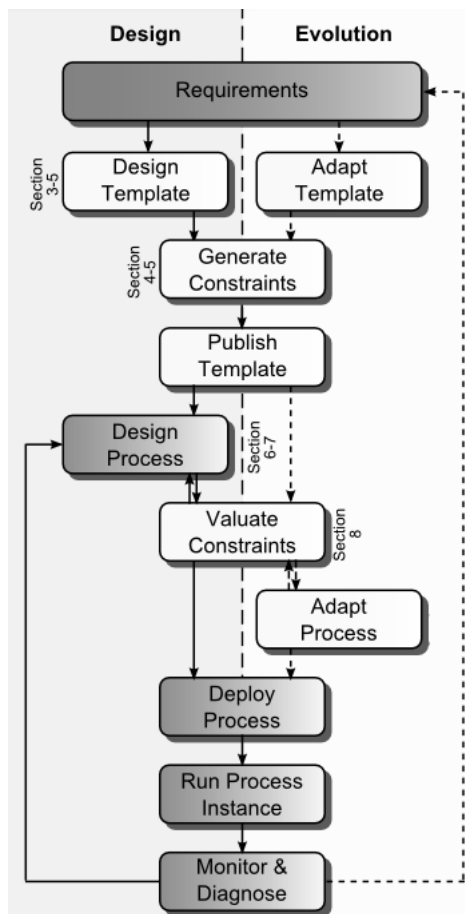
Figure 4: PVDI Engineering Process.
