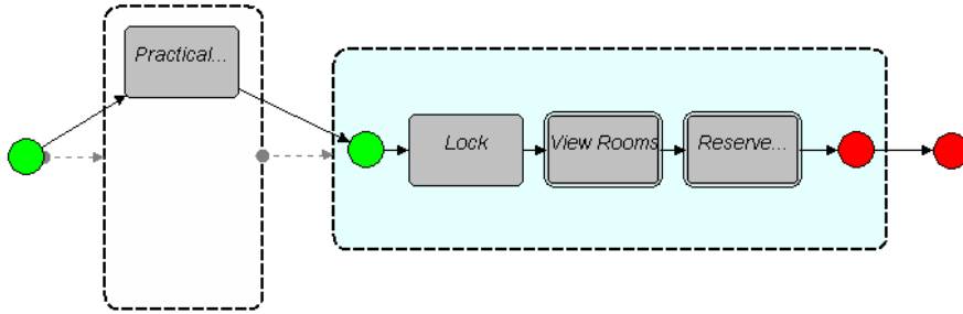
Figure 10: A Valid Variant of Room Reservation Process.
