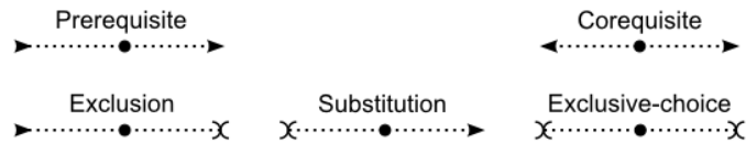
Figure 8: PVDI Graphical Elements for Variation Relations.
