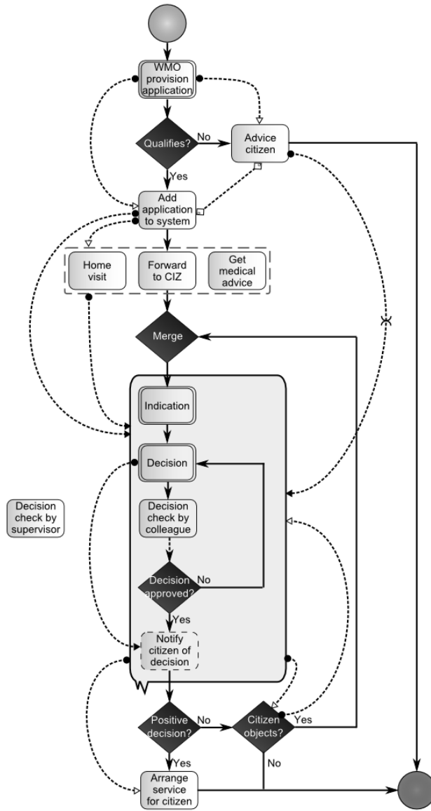
Figure 3: Declarative PVDI view on variability within the WMO processes.
