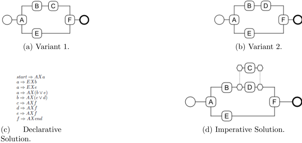
Figure 14: Two variants (a) and (b) and their declarative (c) and imperative (d) solutions.
