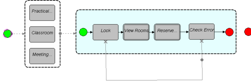
Figure 9: PVDI Room Reservation Template.
