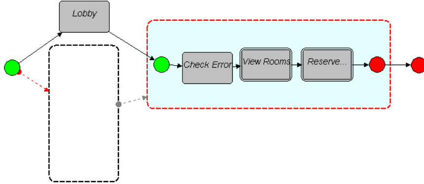
Figure 11: An Example of Invalid Variant for Room Reservation Process.
