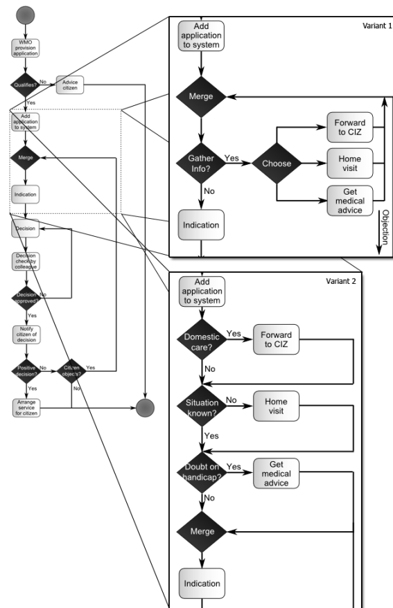
Figure 2: Imperative view on variability within the WMO processes.
