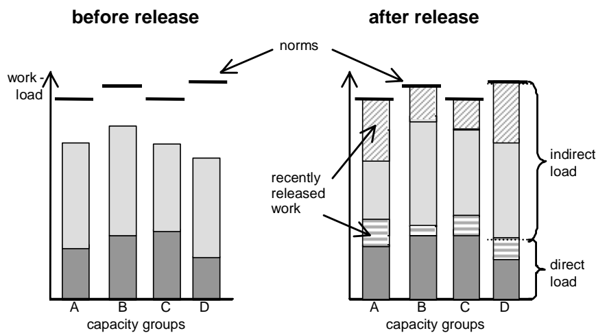
Figure 2.8 Central load balancing
