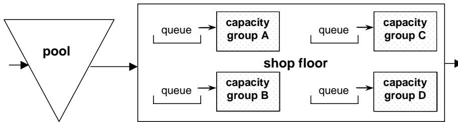
Figure 2.7 Shop floor buffering
