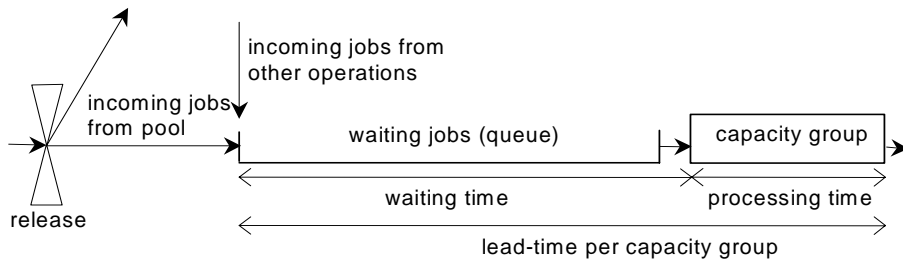
Figure 2.4 Control point at release
