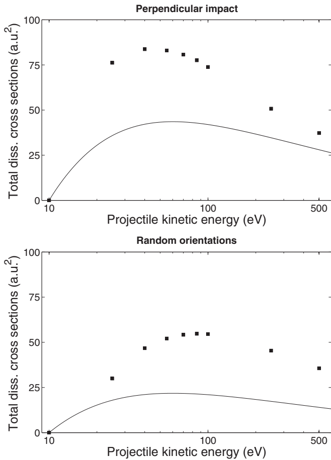
Figure 6. Total anthracene dissociation cross sections after He collisions (squares). The solid line gives the total BCA cross section for collisions leading to excitation energies exceeding T_{\text{co}} = 7.5 eV. For random orientations, the BCA cross section is corrected for orientational averaging to 50% (Micelotta et al. 2010b).
