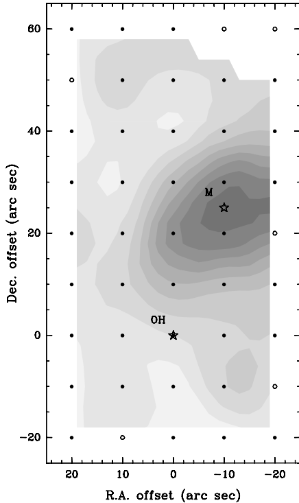
Fig. 1. Distribution of velocity-integrated H 3 O + 364 GHz emission toward Sgr B2, observed with the APEX telescope. Filled dots indicate detections; open dots denote upper limits. The greyscale runs from 1.9 to 35.5 in steps of 3.7 K km s -1 .
