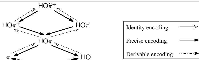
Figure 1 Encodability in Higher-Order Sessions. Precise encodings are defined in Def. 4.6.
