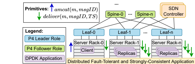
Fig. 1. P4mCast System Architecture.
