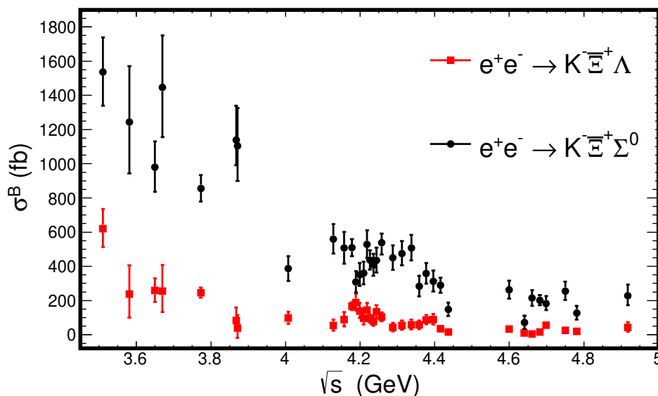
Figure 2. Measured Born cross section for e^+e^- \rightarrow K^- \Xi^+ \Sigma^0 (black) and K^- \Xi^+ \Lambda (red) for each energy point, where the uncertainties include both the statistical and systematic contributions.
