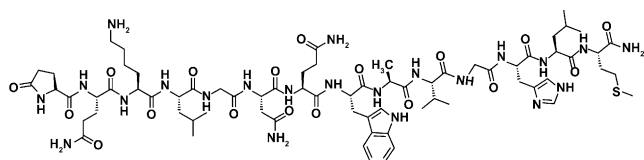
Lys[3]-Bombesin
