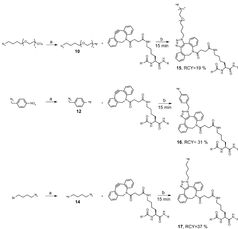
Scheme 4. Reagents and conditions: a) K_2^{18}F , MeCN, 110 °C; b) DMF, RT. R = Pyr-Gln, R 1 = Leu-Gly-Asn-Gln-Trp-Ala-Val-Gly-His-Leu-Met-NH 2 , Pyr = pyroglutamic acid.
