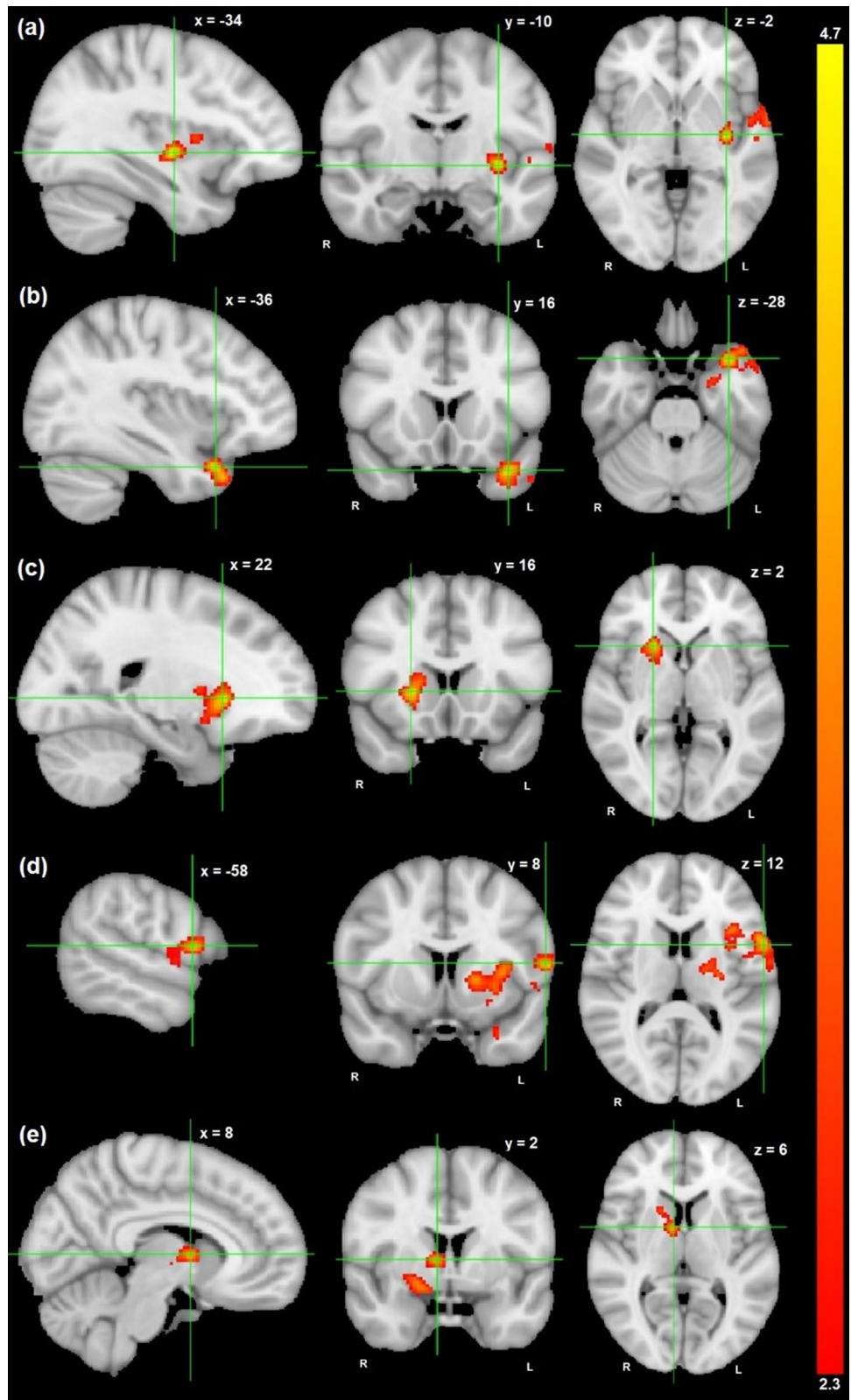
Fig. 1 Brain regions that were (a) negatively correlated with PRS-ADHD at x = -34 , y = -10 , z = -2 during successful inhibition—go, (b-c) positively correlated with PRS-ADHD at x = -36 , y = 16 , z = -28 (b) and at x = 22 , y = 16 , z = 2 (c) during failed inhibition—go, and (d-e) positively correlated with PRS-ADHD at x = -58 , y = 8 , z = 12 (d) and at x = 8 , y = 2 , z = 6 (e) during failed—successful inhibition, shown in radiologic view with the right brain shown on the left. The color bar represents Z-scores (2.3–4.7)
