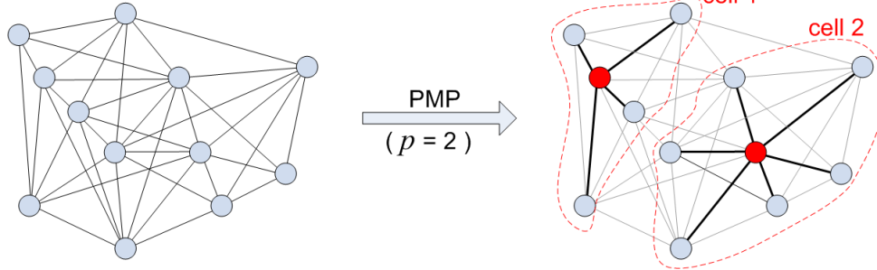
Figure 3.2. The p -Median problem: minimize the total weight of solid edges.
