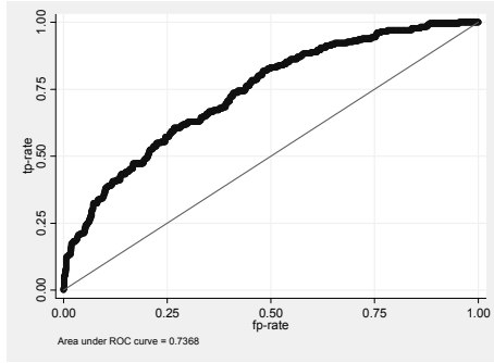
Figure 3.3: ROC-curve
