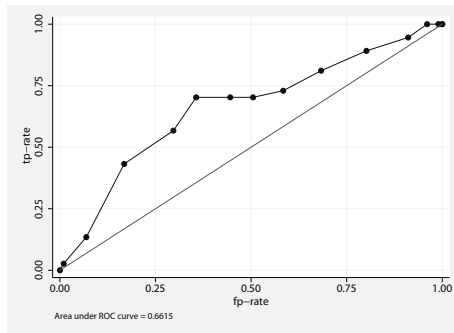
Figure 3.13: ROC-curve
