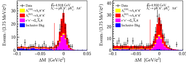
FIG. 3. The distributions of \Delta M for \sqrt{s} = 4.918 (left) and 4.950 GeV (right). The red arrows indicate the cut \Delta M > -0.02 \text{GeV}/c^2 .
