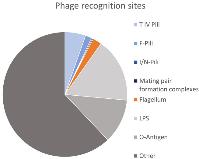
Figure 1. Comparison of recognition sites of bacterial viruses. Pie chart based on the database introduced [13]. Filamentous surface structures are a comparatively rare recognition site (~7.5% of total). As the database does not distinguish between primary and secondary recognition sites, some phages that use different primary and secondary receptors are included twice (once for each receptor).
