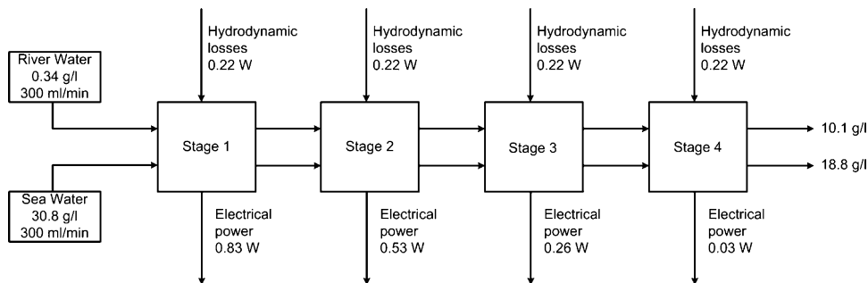
Fig. 7. In- and out-going potential salinity power, the delivered electric power and the hydrodynamic losses in a four stage experiment with a 50 cell stack with a total membrane area of 1 \text{ m}^2 .
