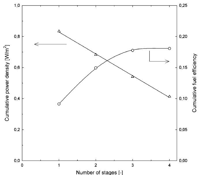
Fig. 9. Cumulative power density and cumulative gross energy efficiency of a system with 1, 2, 3 and 4 stages.
