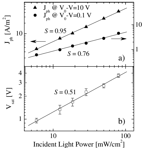
FIG. 4. (a) Incident light power (ILP) dependence of the photocurrent J_{ph} taken from Fig. 3 at an effective voltage of V_0 - V = 0.1 V and V_0 - V = 10 V (symbols). (b) Saturation voltage ( V_{sat} ) versus ILP as determined for Fig. 3. The slope ( S ) determined from the linear fit (solid lines) to the experimental data is written on the figure.
