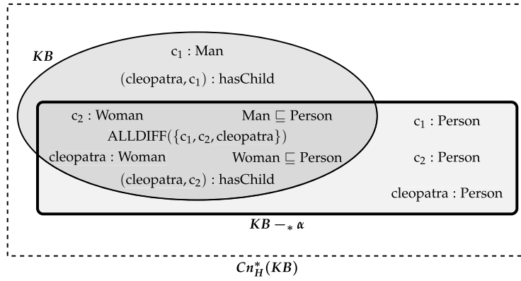
Fig. 4. Cn_H^* in Example 33.
