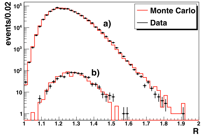
Fig. 2. Distributions of the number of events as a function of the R energy estimator for data and MC before the second-level cut. a) downgoing muons; b) mis-reconstructed as upgoing muons. The points are 12 line data, the histograms show the atmospheric muon MC normalized to the data.
