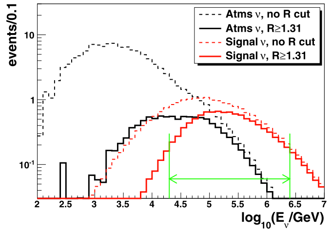
Fig. 4. Signal and background neutrino energy spectra as a function of the true neutrino energy after the second-level cut with and without the requirement R \geq 1.31 . The energy region containing 90% of the astrophysical neutrino signal is indicated.
