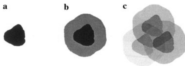
Figure 5. (a) 2D example of a body M , (b) the contact body N of M , (c) N used to construct a situation where three copies of M touch each other. Notice that N is point-symmetric.
