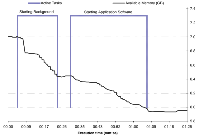
Figure 4. Example of task resource usage model
