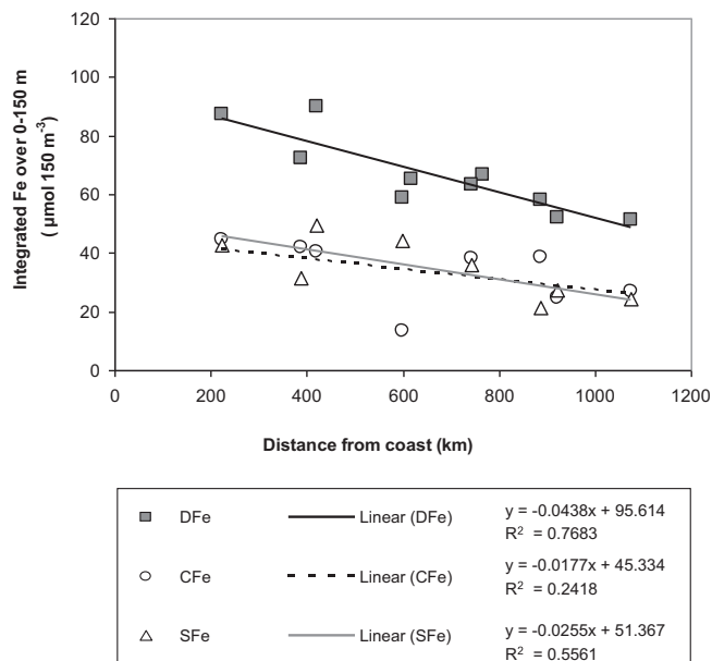
Fig. 7. Relationship between integrated concentrations of DFe, CFe and SFe from casts (0–150 m) and distance from the North West African coast.
