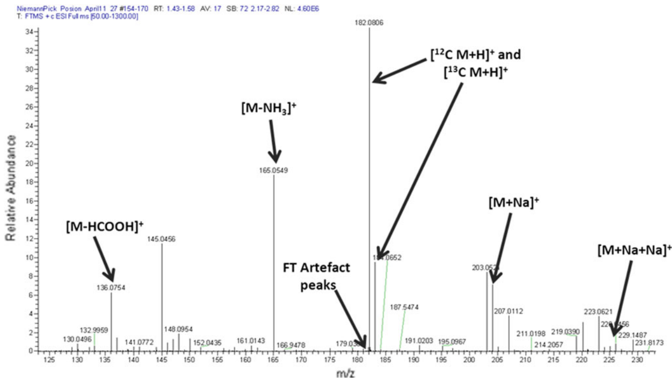
Fig. 4 Full-scan mass spectrum related to the detection of tyrosine on a UPLC–MS system (Waters Acquity UPLC system coupled to a ThermoFisher LTQ-Orbitrap XL hybrid mass spectrometer). The complex array of ion types detected includes loss of formate and
