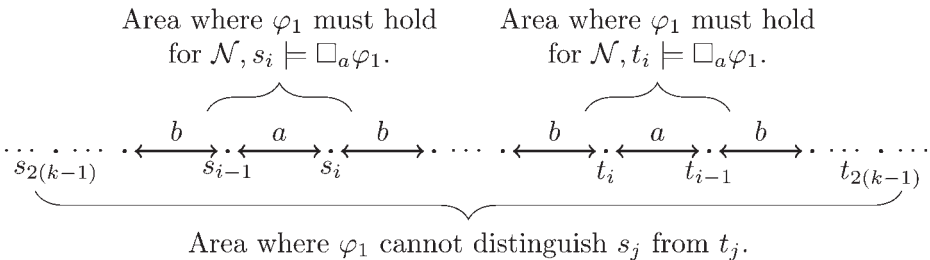
Fig. 2. The formula \varphi = \Box_a \varphi_1 cannot distinguish between s_i and t_i , since \mathcal{N}_n, w_i \models \varphi \Leftrightarrow (\mathcal{N}_n, w_i \models \varphi_1 \text{ and } \mathcal{N}_n, w_{i-1} \models \varphi_1) for w \in \{s, t\} , and by the induction hypothesis \varphi_1 cannot distinguish either s_i from t_i or s_{i-1} from t_{i-1} .
