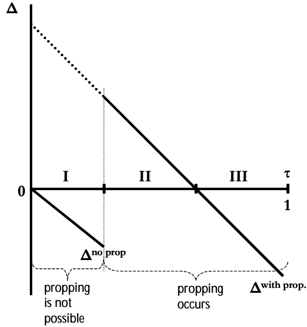
Figure 3: The relationship between \tau and \Delta^*
