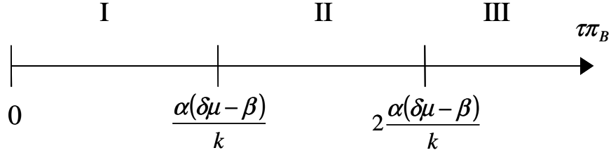
Figure 1: Critical values for the (maximum) amount to be tunneled.
