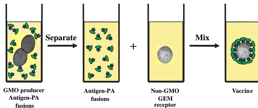
Fig. 1. Production of a vaccine: binding of PA fusions to GEM particles. In a two-step procedure, antigens containing a protein anchor domain (PA) and a gram-positive enhancer matrix (GEM) particle of bacterial origin are used to make a vaccine. First, the antigen–PA fusions are produced in the medium and separated from the producer cells. Next, GEM particles and cell-free medium are mixed. The PA directs the antigens to the surface of the GEM particles, where they bind tightly to the peptidoglycan layer.
