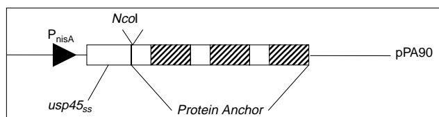
Fig. 2. The pPA90 vector. Schematic representation of a part of the general display vector pPA90. Abbreviations: P nisA , inducible nisA promoter; usp45 ss , usp45 signal sequence; NcoI , restriction site for integration of antigen genes; hatched blocks depict the LysM repeat sequences.
